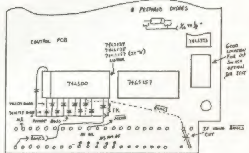
Illustration F: Stack of ICs & Signal Locations
